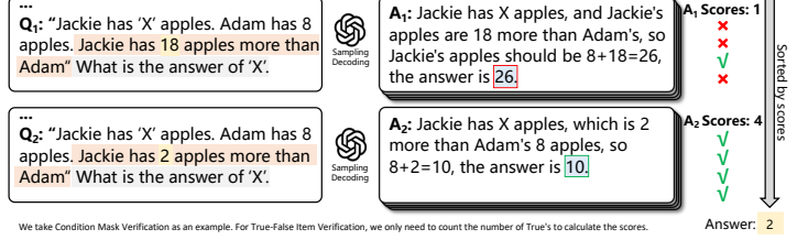
Figure 2: Example of self-verification. In the step one, LLM generates candidate answers and forms different conclusions. Then, in the step two, LLM verifies these conclusions in turn and computes the verification score.
